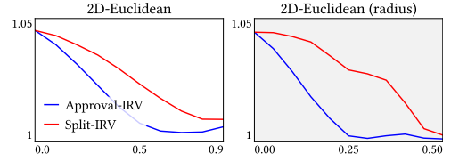
Fig. 17. Average distortion of the winner.
