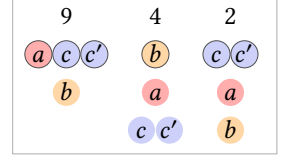
Fig. 9. Split-IRV fails independence of clones.
