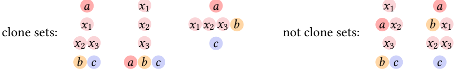
Fig. 8. Examples of X = \{x_1, x_2, x_3\} being a clone set or not being a clone set.
